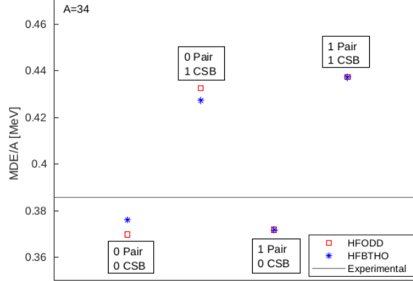
Figure 4.5: Comparison of MDE/A between the experimental results (black line), HFODD results (red squares) and HFBTHO results (blue asterisks) for the mirror nuclei ^{34}\text{S} - ^{34}\text{Ar} .
