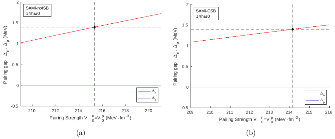
Figure 4.3: Same of the figure 4.2, but for 14 shells. V_0 = -215.327 [MeV·fm -3 ] in the panel (a) and V_0 = -214.151 [MeV·fm -3 ] in the panel (b).
