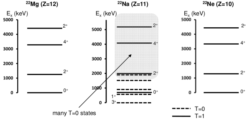
Figure 3.2: Level structure in the A = 22 isospin triplet [36].
