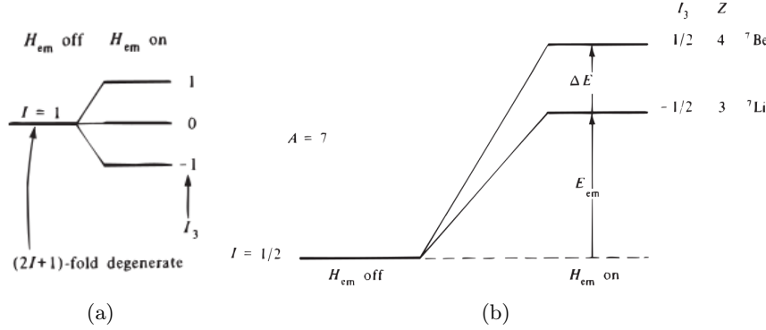
Figure 3.1: Effect of electromagnetic interaction on the isospin multiplet T (in both the figures indicated as I , whereas T_z is indicated as I_3 ). Panel (a) shows how electromagnetic interaction breaks the (2T + 1) -fold degenerate state. Panel (b) reports the specific example of the effect of electromagnetic interaction on the A = 7 isospin doublet. It lifts and breaks the degenerate state into two sub-states [30].
