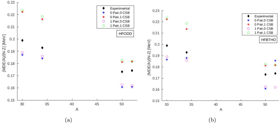
Figure 4.8: Comparison of (\text{MDE}/A)/|N-Z| [MeV] calculated with HFODD in panel (a) and calculated with HFBTHO in panel (b). The black filled diamond indicates the experimental value
