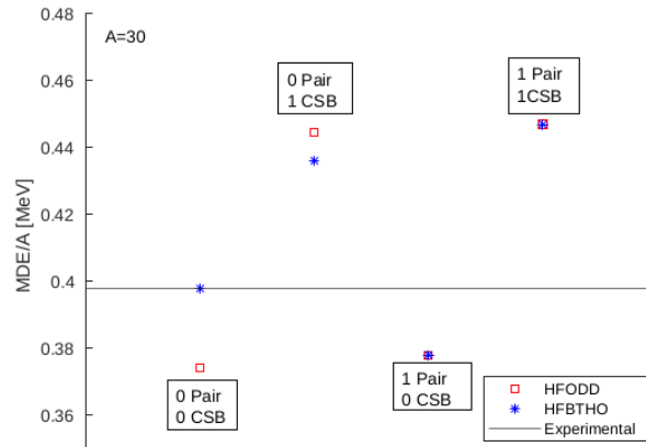
Figure 4.4: Comparison of MDE/A between the experimental results (black line), HFODD results (red squares) and HFBTHO results (blue asterisks) for the mirror nuclei ^{30}\text{Si} - ^{30}\text{S} .
