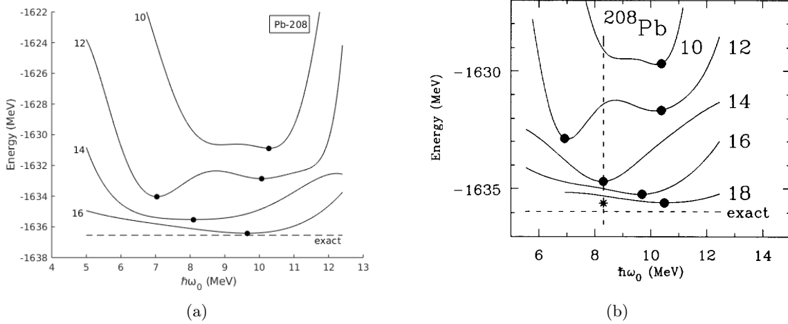
Figure B.1: Ground-state energies of ^{208}\text{Pb} calculated as functions of \hbar\omega_0 for several values of the number N_0 of HO shells included in the basis. Dots denote the minima. The horizontal dashed line represents the exact result. In the (b) panel the same calculation made by Dobaczewski et al. [23, 24] is reported.
