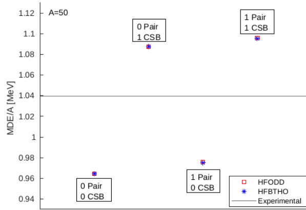
Figure 4.6: Comparison of MDE/A between the experimental results (black line), HFODD results (red squares) and HFBTHO results (blue asterisks) for the mirror nuclei ^{50}\text{Ti} - ^{50}\text{Ni} .
