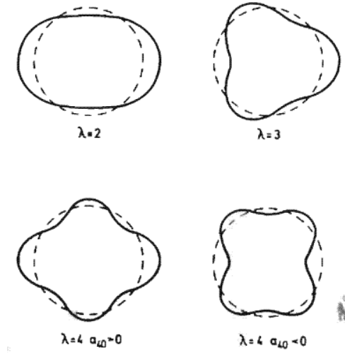
Figure 1.3: Nuclear shapes with quadrupole \lambda = 2 , octupole \lambda = 3 and hexadecupole \lambda = 4 deformations [44]
