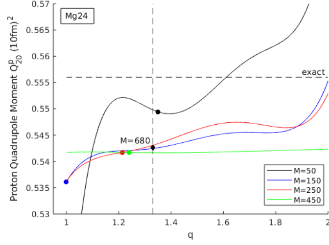
Figure B.3: Same as in figure B.2 but for proton quadrupole moments of ^{24}\text{Mg} . The horizontal dashed line represents the exact result.
