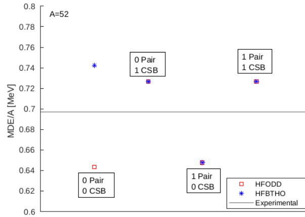
Figure 4.7: Comparison of MDE/A between the experimental results (black line), HFODD results (red squares) and HFBTHO results (blue asterisks) for the mirror nuclei ^{52}\text{Cr} - ^{52}\text{Ni} .
