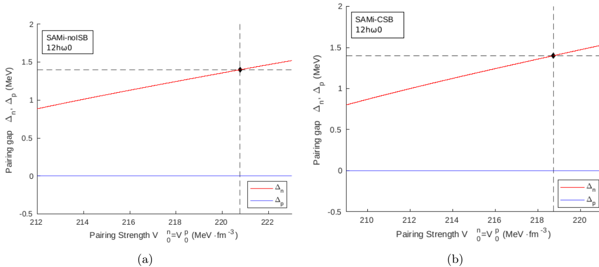
Figure 4.2: Trend of the proton ( \Delta_p ) and neutron ( \Delta_n ) pairing gap as a function of |V_0| for ^{120}\text{Sn} . Filled diamonds indicate the value of V_0 for which \Delta_n = 1.4 MeV, that are V_0 = -220.778 [\text{MeV} \cdot \text{fm}^{-3}] in the panel (a) and V_0 = -218.715 [\text{MeV} \cdot \text{fm}^{-3}] in the panel (b). Calculation performed with 12 shells.
