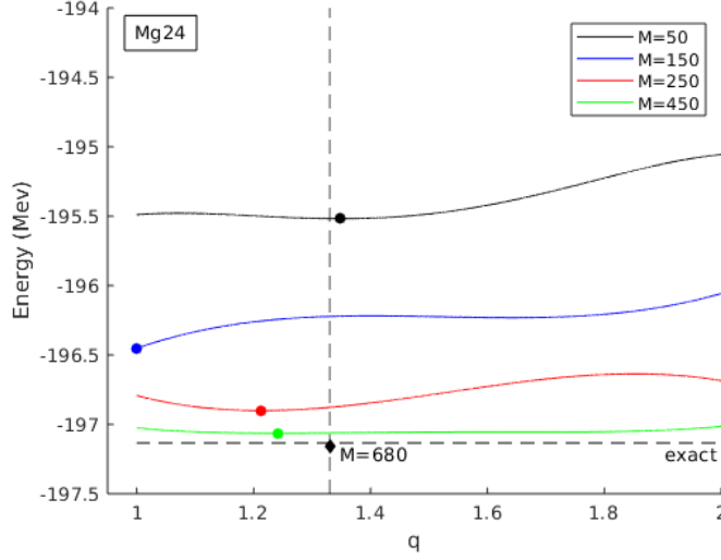
Figure B.2: Energies of ^{24}\text{Mg} (solid lines) calculated as functions of the basis deformation parameter q , \hbar\omega_0 = 14.214 MeV fixed and for several values of the number M states included in the HO basis. Dots denote the minima. The horizontal dashed line represents the exact result.
