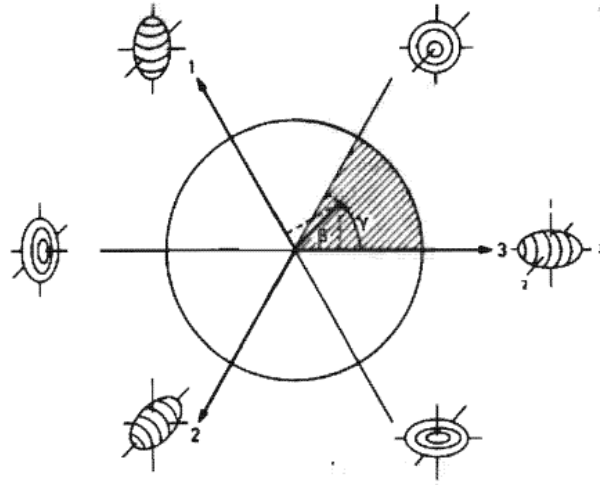
Figure 1.4: Quadrupole nuclear shapes in the \beta - \gamma plane [44].
