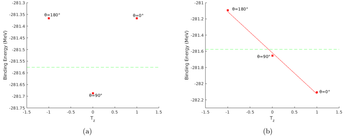
Figure 4.1: Calculated ground-state energies of the A=30 isospin-triplet nuclei. Calculations were performed with Skyrme parameter set SV [44] and without Coulomb interaction and without pairing. Full red squares in the (a) and (b) panels show the results obtained by adding only the class II and the class III forces, respectively. The dashed green line indicates the ground state energy without any ISB terms included. The parameters t_0 and x_0 has been set with the values t_0^{\text{II}} = 20 \text{ MeV}\cdot\text{fm}^3 , t_0^{\text{III}} = -8 \text{ MeV}\cdot\text{fm}^3 , x_0^{\text{II}} = x_0^{\text{III}} = 0 , as indicated in [4]
